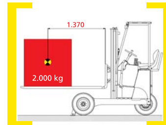
2.000 kg at 1.370 mm LSP
