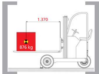
876 kg at 1.370 mm LSP
