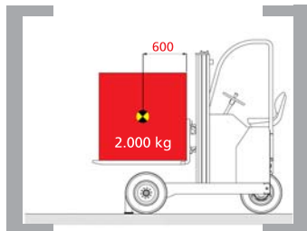
2.000 kg at 600 mm LSP
